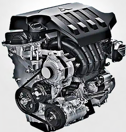
1.5L Engine with MIVEC Maximum Power 105 Ps / 6000 rpm
